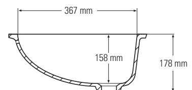
Side cross-section
